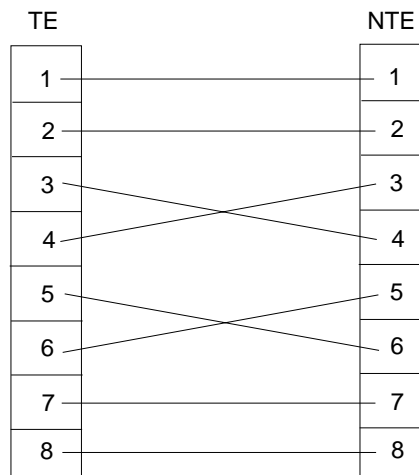
Figure B-1 ISDN Terminal Endpoint Connector
